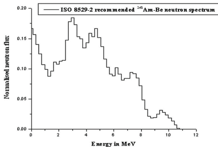
Figure 1: Neutron energy spectrum of Am-Be source
