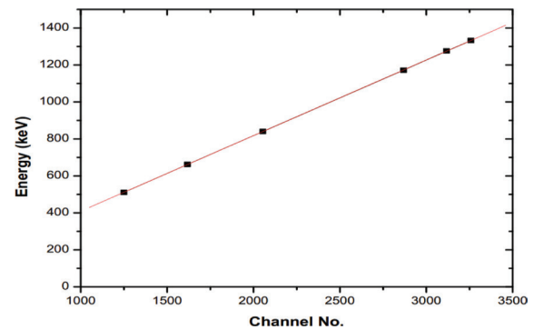
Figure 3: Calibration curve of HPGe detector
