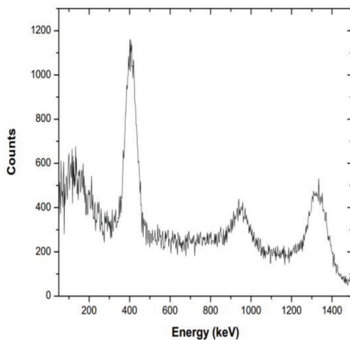
(b) The spectrum of 115 In with Cd foil irradiation
