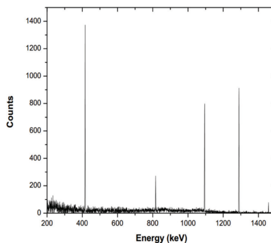
(b) The spectrum of 115 In with Cd foil irradiation
