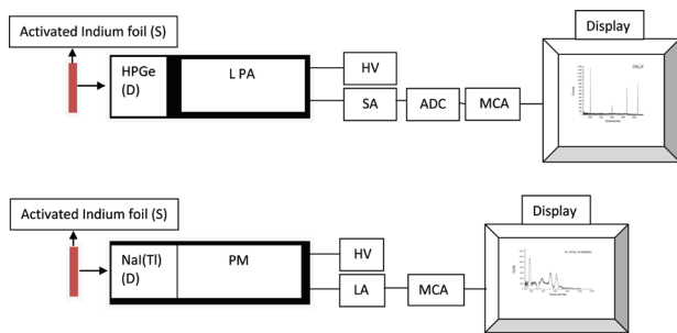
Figure 2: Experimental arrangements
