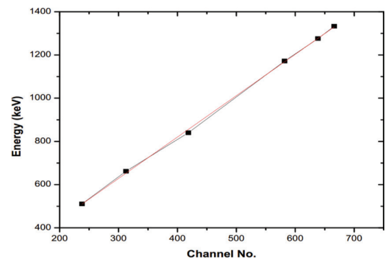
Figure 4: Measurements using HPGe detector
