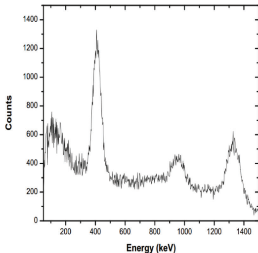
(a) The spectrum of 115 In without Cd foil irradiation
