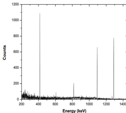
(a) The spectrum of 115 In without Cd foil irradiation
