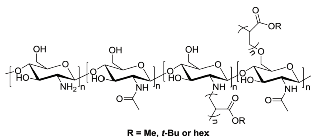
Figure 4: Structure of chitosan-g-polyacrylate.
